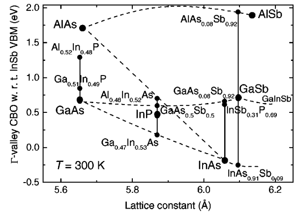
FIG. 12. Conduction band offsets corresponding to the VBOs in Fig. 11. The various points and curves have the same meaning as in that figure.
